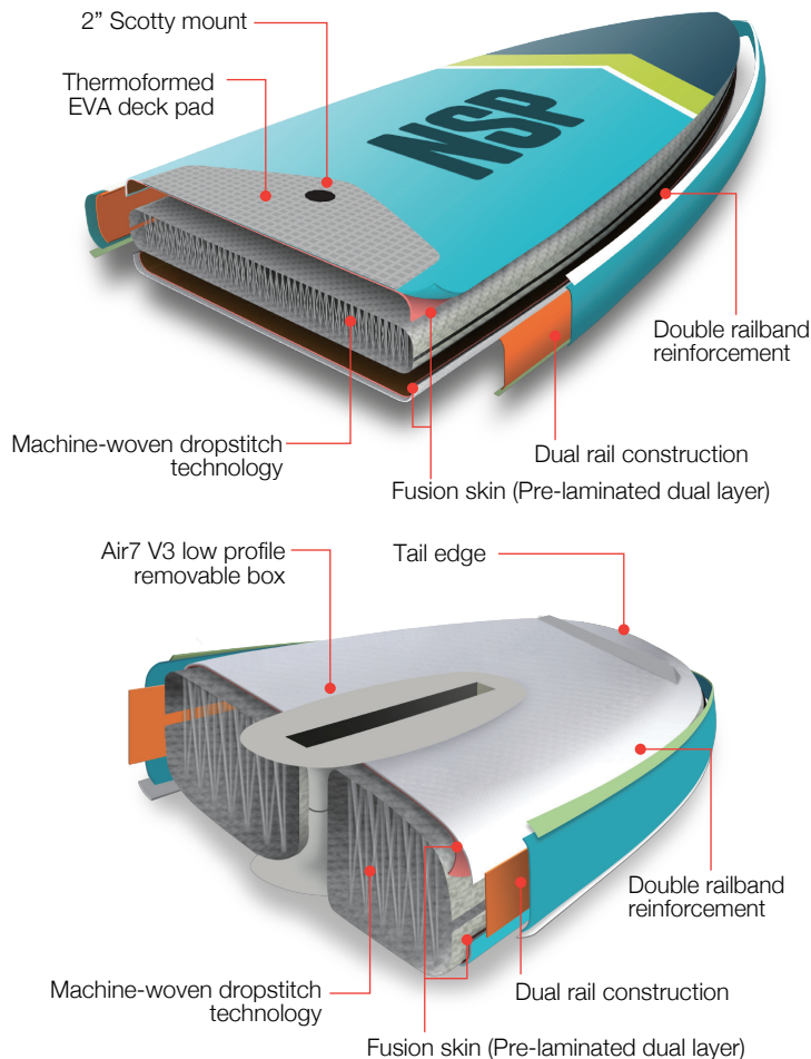
Fusion-reinforced double layer glueless pre-lamination
